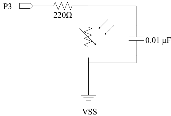
Photoresistor
