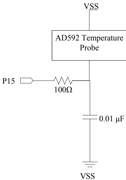
Temperature Probe
